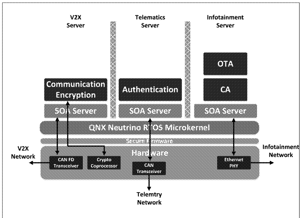
Figure 6. Remote management server software architecture
