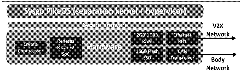
Figure 9. Example security server ECU architecture
