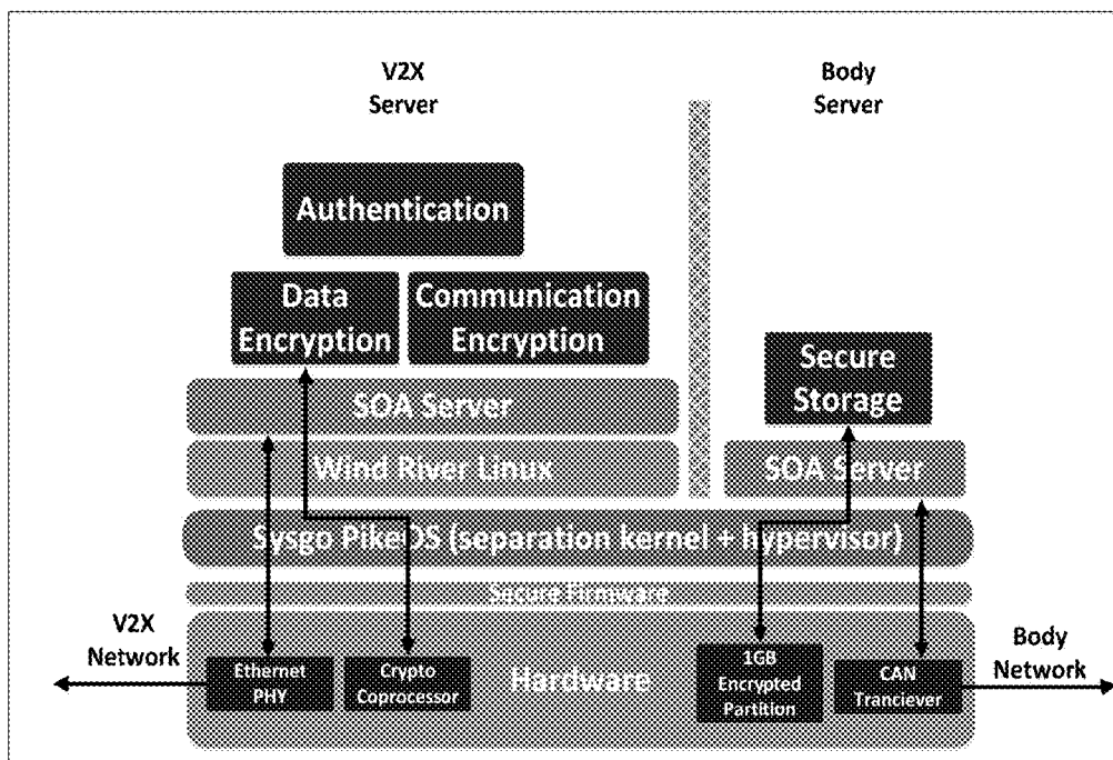
Figure 10. The inventive SOA security server architecture example
